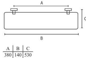
Porta Shampoo Grade
