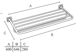
Porta Toalha Rack
